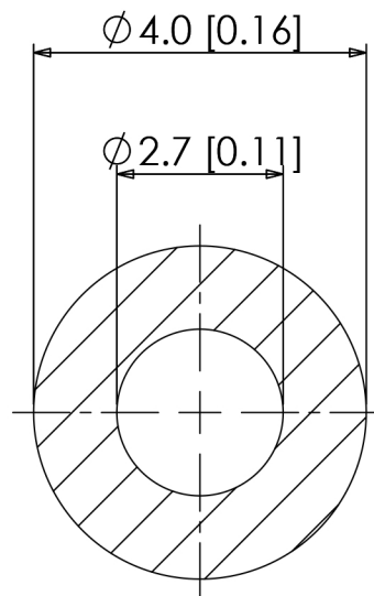
CROSS SECTION OF HOSE
